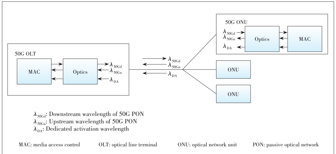
▲ Figure 4. Dedicated activation wavelength for 50G PON
