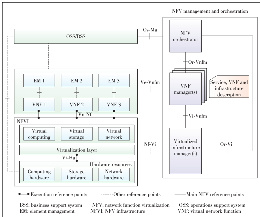
▲ Figure 5. NFV architecture [19].
